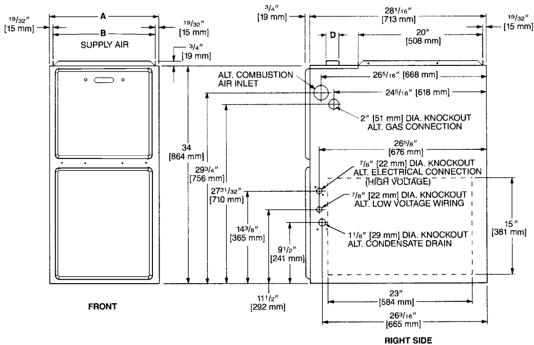
RIGHT SIDE
